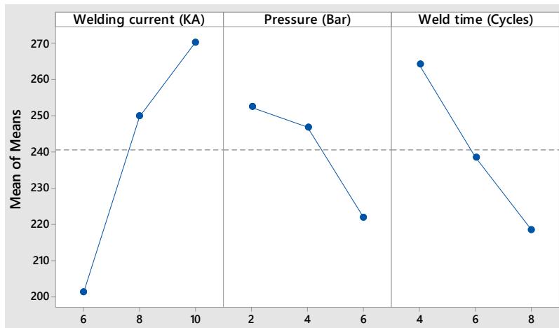
Fig. 26 Main effects plot for means
