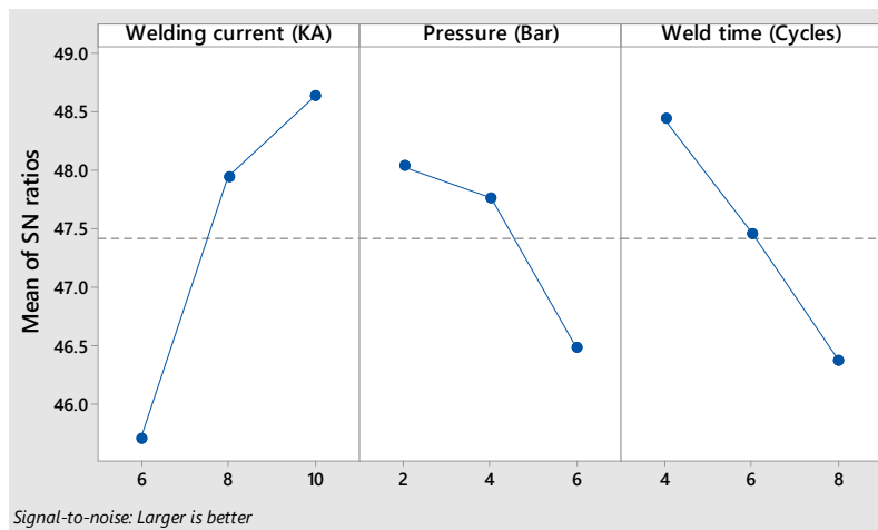
Fig. 27 Main effects plot for SN ratios
