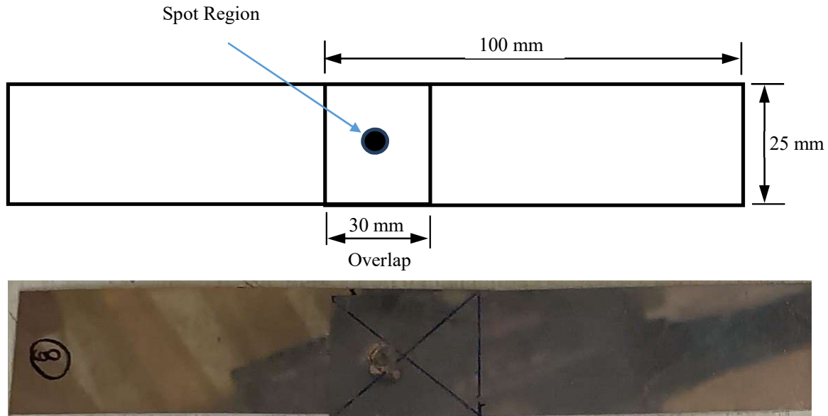
Fig. 2 Sample Specimen
