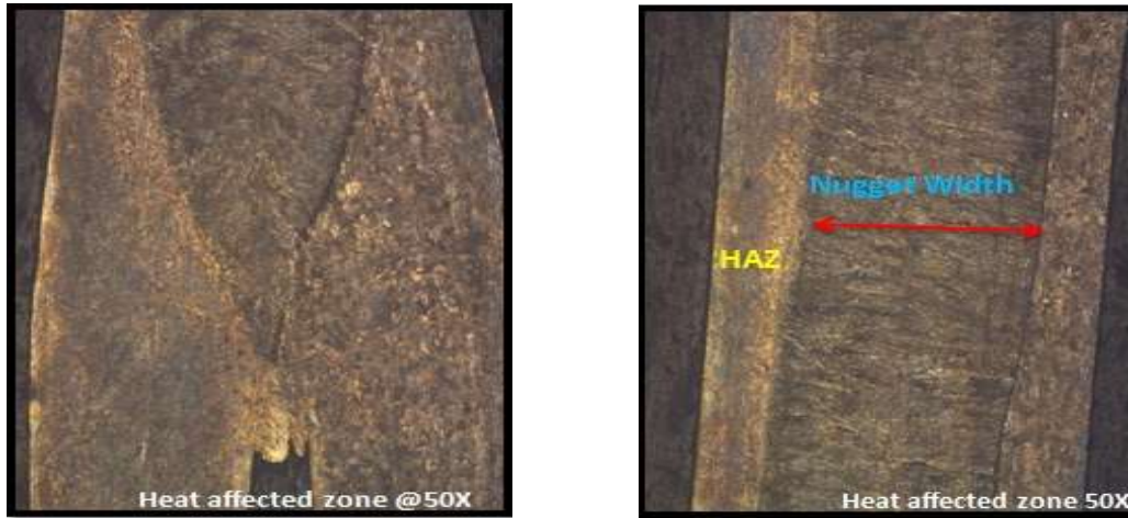
Fig. 21 and Fig. 22 Microstructure for weld zone and heat affected zone for sample 8 At 50X magnification
