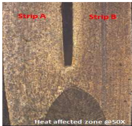
Fig. 11 Weld zone for sample 1 @ 50x
