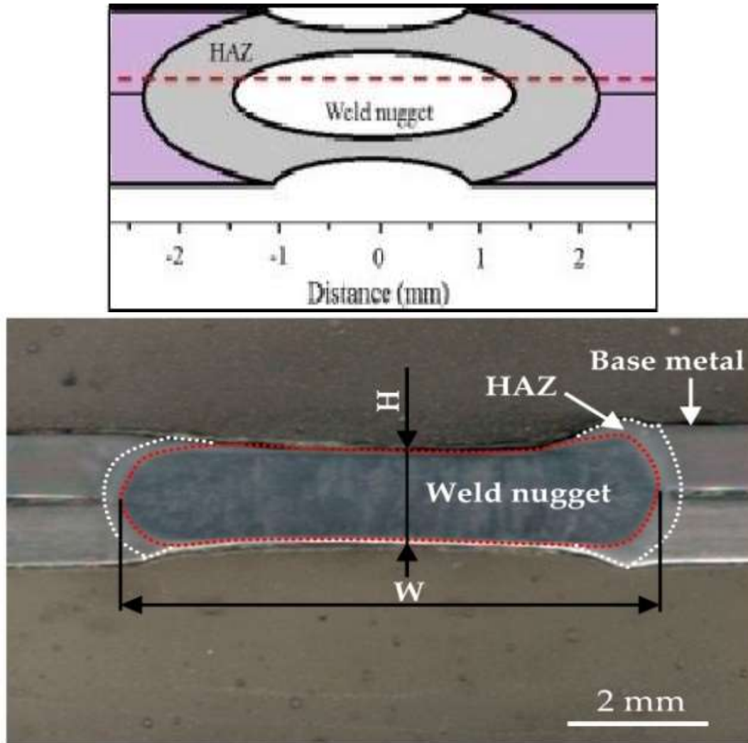
Fig. 9 Weld zone
