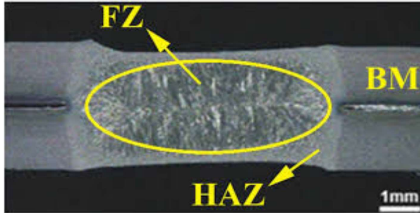
Fig. 10 Weld attributes revealed by metallographic sectioning.
